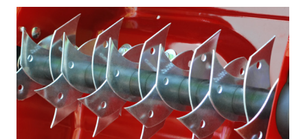
The Cobra S390H petrol Scarifier comes equipped with 16 fixed steel blades.
